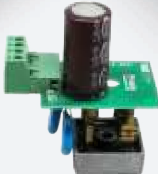
3300 µF KONDANSATÖRLÜ KÖPRÜ DİYOT KARTI (35A) BRIDGE DIODE CARD WITH 3300 µF CAPACITOR (35A)
